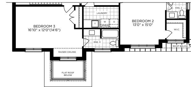
PARTIAL SECOND FLOOR PLAN ELEV. C
