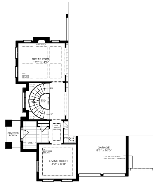
PARTIAL GROUND FLOOR PLAN ELEV. C
