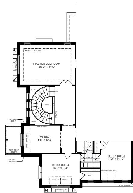
PARTIAL SECOND FLOOR PLAN ELEV. B
