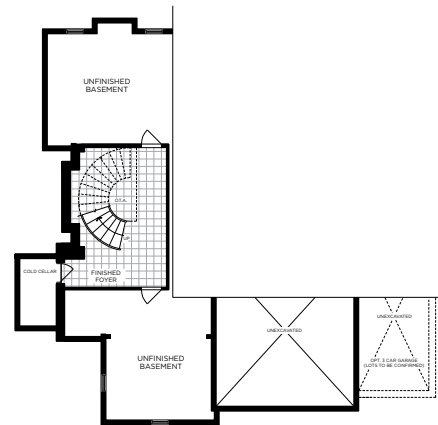
PARTIAL BASEMENT PLAN ELEV. C
