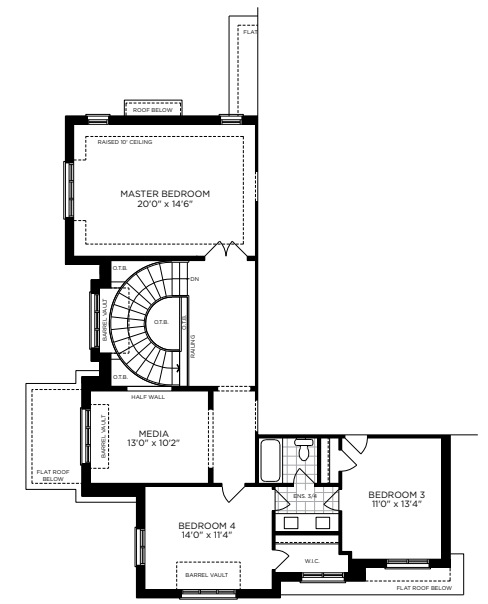
PARTIAL SECOND FLOOR PLAN ELEV. C
