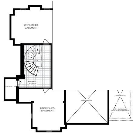
PARTIAL BASEMENT PLAN ELEV. B
